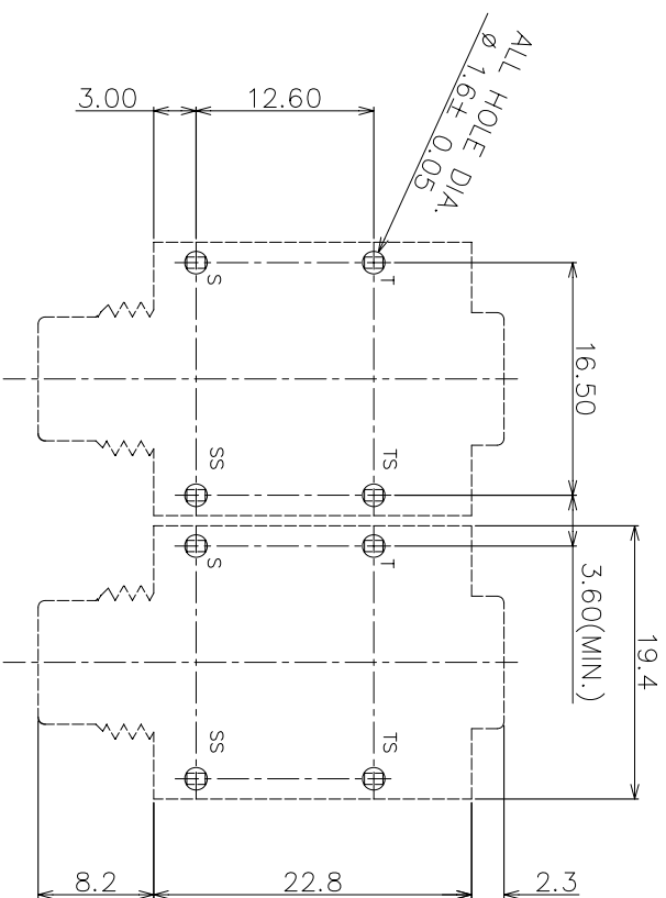
PCB LAYOUT
