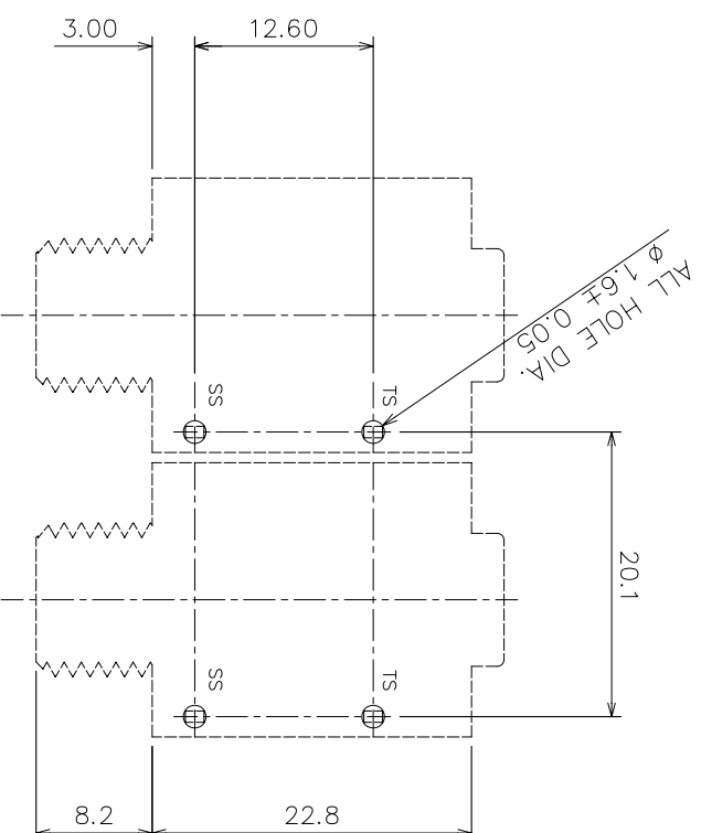
PCB LAYOUT
